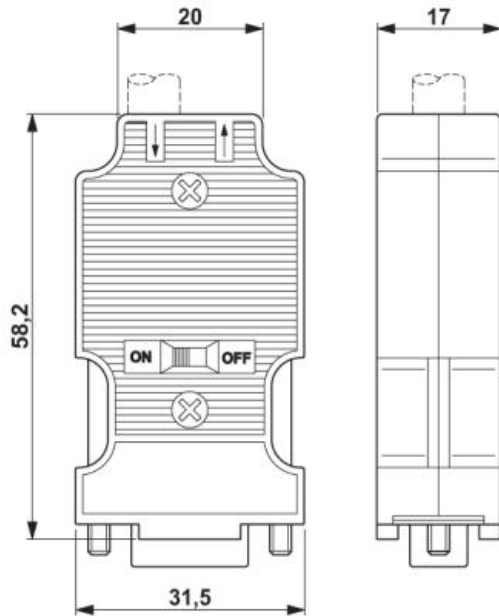
Dimensional drawing SUBCON-PLUS- PROFIB/AX/SC
